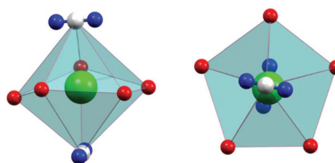
Fig. 2 The side and top view of the DPB polyhedron of 8 . Colour codes: Dy, bright green; N, blue; O, red; centroid of N–N, white.
