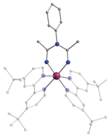
Fig. 2 The molecular structure of the cationic complex 2 . 41 For clarity reasons H-atoms, disorder conformers and lattice counter ions have been omitted, as well as partial transparency has been employed. Colour code: C: grey, N: blue, Rh III : purple. Reproduced using reported cif.
