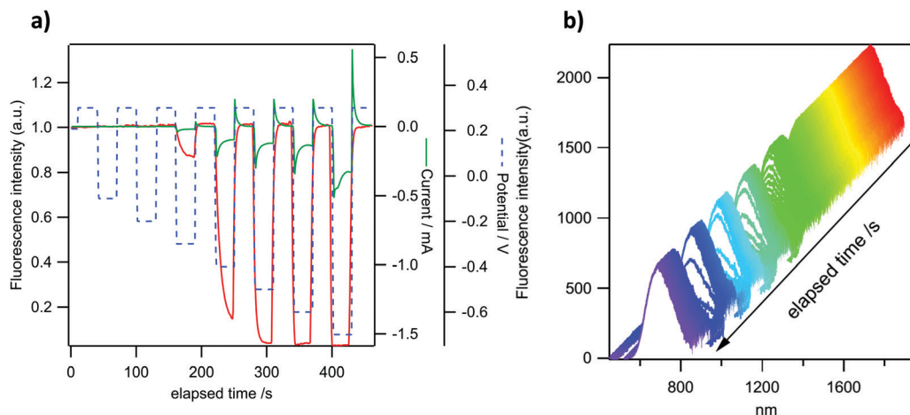
Fig. 10 Modulation of fluorescence intensity (red trace) and electrochemical current (green trace) of compounds 8 2+ (a) for potential steps of increasing amplitude (dashed blue trace). (b) Corresponding variation of emission spectra with time of compound 8 2+ for the same potential signal as in (a).
