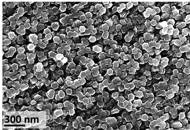
Fig. 7 SEM image of zinc substrate after exposure to [C_4C_{1im}]Cl (IL-1, X_{H_2O} = 0.75 solution, 20 \pm 1 °C) for 26 d, showing the top of hexagonal nanorods (average size 150 \pm 30 nm, n = 278 ).
