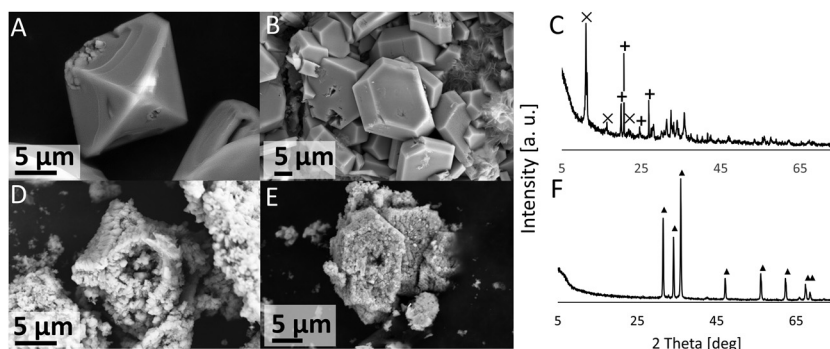
Fig. 6 SEM images of the ZnO precursors formed in the zinc surface exposed to [C_4C_1im]Cl (IL-1, X_{H_2O} = 0.98 solution, 20 \pm 1^\circ C and 44 d) before and after calcination. \epsilon -Zn(OH) _2 octahedrons before (A) and after calcination (D). ZHC particles before (B) and after (E) calcination. Both \epsilon -Zn(OH) _2 and ZHC are transformed to ZnO with overall conservation of the morphology with increased porosity. XRD spectra of the \epsilon -Zn(OH) _2 and ZHC powder before (C) and after calcination (F). Main peaks from diffraction patterns had been labelled: (x) ZHC, (+) \epsilon -Zn(OH) _2 and ( \blacktriangle ) ZnO.
