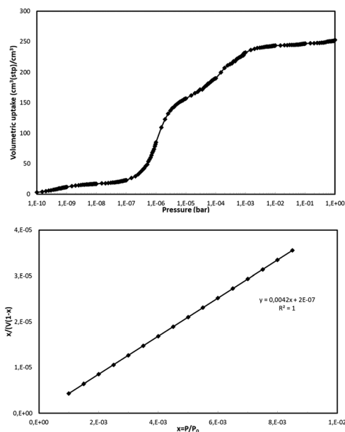
Fig. 12 N 2 volumetric uptake isotherm at 77 K for the calculation of the BET surface area of NUIG1 (top), and plot of the selected linear region that satisfies the consistency criterion (bottom). 48
