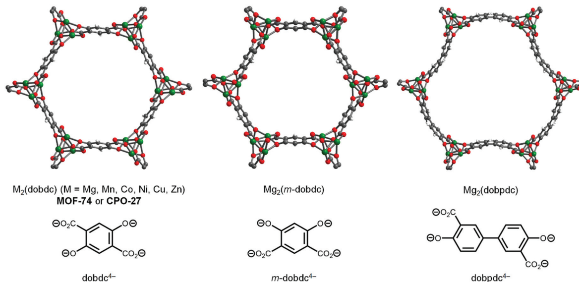
Fig. 1 Structures of the open metal site metal–organic frameworks M_2(\text{dobdc}) ( M = \text{Mg, Mn, Co, Ni, Cu, Zn} ; \text{dobdc}^{4-} = 2,5\text{-dioxidobenzene-1,4-dicarboxylate} ), Mg_2(m\text{-dobdc}) ( m\text{-dobdc}^{4-} = 2,4\text{-dioxidobenzene-1,5-dicarboxylate} ), and Mg_2(\text{dobpdc}) ( \text{dobpdc}^{4-} = 4,4'\text{-dioxidobiphenyl-3,3'-dicarboxylate} ). The cross-pore diameters in these MOFs are 15.4 Å, 14.9 Å, and 22.8 Å, respectively. Gray, white, red, and green spheres represent carbon, hydrogen, oxygen, and magnesium, respectively.
