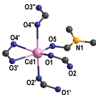
Fig. 3 Coordination environment of cadmium(II) in \{[\text{Cd}(\text{L})(\text{DMF})]\cdot\text{DMF}\}_n (2). Hydrogen atoms and non-coordinating DMF are omitted for clarity.
