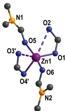
Fig. 2 Coordination environment of zinc(II) in \{[\text{Zn}(\text{L})(\text{DMF})_2]\}_n (1). Hydrogen atoms and non-coordinating DMF are omitted for clarity.
