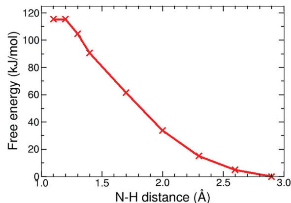
Fig. 9 Free energy profile of the protonation reaction, 1 2- + H + → 1H - , in acetonitrile computed with constrained DFT-MD simulations.
