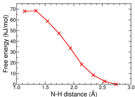
Fig. 8 Free energy profile of the protonation reaction, 1 - + H + → 1H , in acetonitrile computed with constrained DFT-MD simulations.
