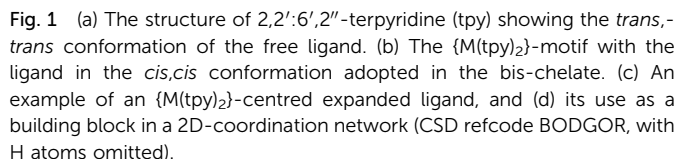
realism of coordination polymers and networks requires functionalization of the tpy ligand by a second metal-binding domain such as a heterocycle or carboxylate to produce an \{M(\text{tpy})_2\} -centred 'expanded ligand'. 5 An example is shown in Fig. 1c, and reaction of this complex with \text{CuCl}_2 \cdot 2\text{H}_2\text{O} yields a 2D-network \{[\text{Ru}(4'\text{-pymtpy})_2][\text{CuCl}_2(\text{OH}_2)][\text{CuCl}_3\text{Cl}]\}_n (4'-pymtpy = 4'-(5-pyrimidinyl)-2,2':6',2''-terpyridine), part of which is shown in Fig. 1d. 6 Fortunately, functionalization in the 4'-position of tpy is readily accomplished using either Wang and Hanan's one-pot strategy 7 or the Kröhnke methodology. 8 On occasion, cyclic products (easily recognized from their ^1\text{H} NMR spectroscopic signatures compared to that of a tpy) result for particular 4'-substituents; the reasons for this remain unclear. 9
