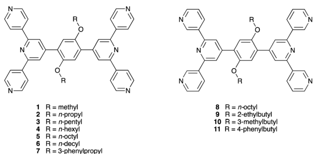
Scheme 4 Structures of tetrapotic ligands with 4,2':6',4'' -tpy domains (left) and 3,2':6',3'' -tpy domains (right).
