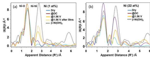
Fig. 3 Ni EXAFS spectra acquired under dry, OC potential and OER potential (+1.56 V) conditions using (a) 1% Ni ( \beta -FeOOH:Ni) and (b) 22% Ni ( \beta -FeOOH:Ni) surface-decorated with \text{Ni}(\text{OH})_2 together with that of the reference compound \beta -Ni(OH) _2 .
