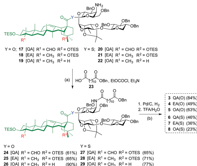
Scheme 2 Reagent and conditions: (a) EtOCOCI, \text{Et}_3\text{N} , THF, 0 °C to r.t., 4 h, 61% (for 24), 65% (for 25), 90% (for 26); 65% (for 27), 71% (for 28), and 77% (for 29); (b) 1: Pd/C, \text{H}_2 (1 atm), EtOH/THF 1 : 1, r.t., 16 h (for 24–26); 20 min (for 27–29); 2: TFA/ \text{H}_2\text{O} 3 : 1, 0 °C, 1 h, 84% (for 3), 49% (for 4), 63% (for 5); 46% (for 6), 36% (for 7), and 23% (for 8).
