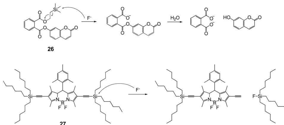
Fig. 11 Reaction schemes of 26 and 27 with F − .
