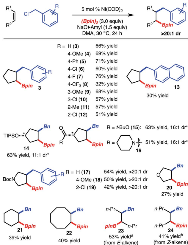
Scheme 3 Substrate scope.
