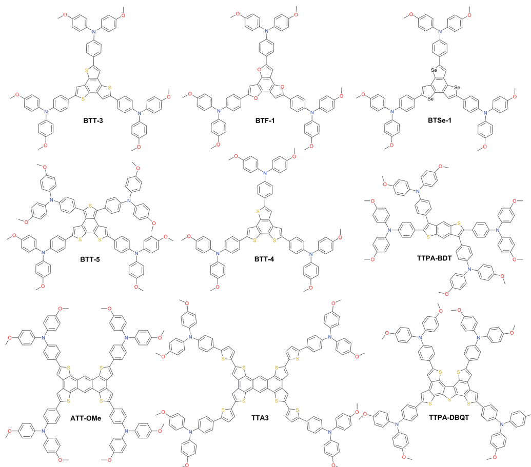
Fig. 11 Chemical structures of the most efficient hole transporting materials based on benzodithiophene (BDT), benzotrithiophene (BTT), benzotrifuran (BTF), benzotriselenophene (BTSe), anthratetrathiene (ATT), and dibenzoguinethiophene (DBQT) cores.
