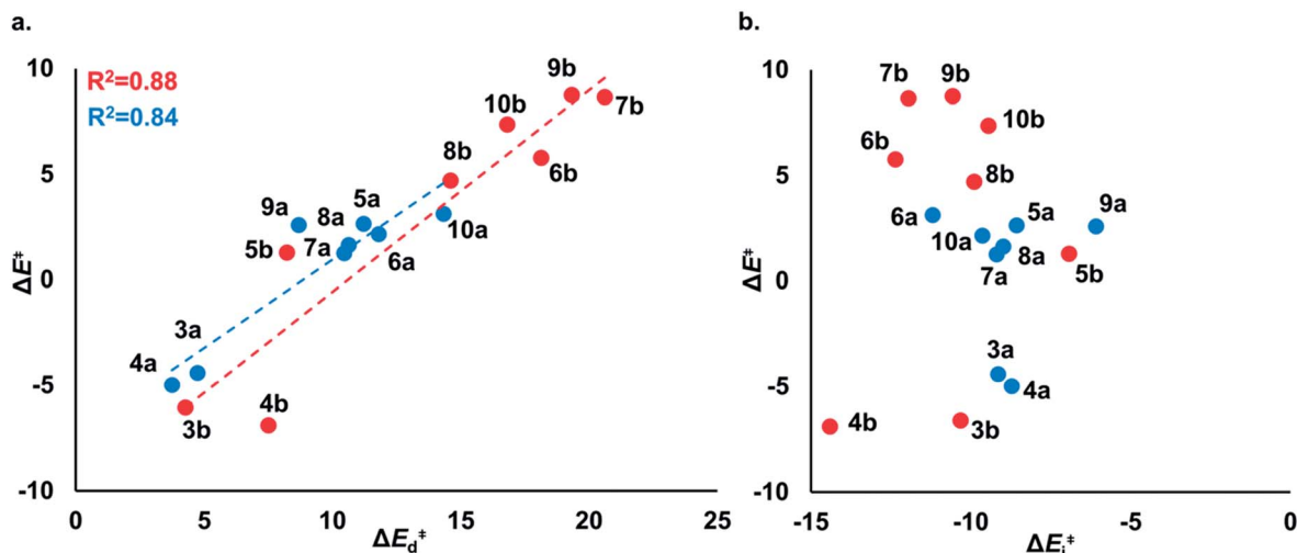
Fig. 4 (a) \Delta E^\ddagger vs. \Delta E_{\text{d}}^\ddagger of the nucleophilic addition of \text{MeS}^- towards cyclic thiosulfates (blue) and cyclic disulfides (red). The linear equation for (3–10)a is \Delta E^\ddagger = 0.84\Delta E_{\text{d}}^\ddagger - 7.40 . The linear equation for (3–10)b is \Delta E^\ddagger = 0.96\Delta E_{\text{d}}^\ddagger - 10.12 . (b) \Delta E^\ddagger vs. \Delta E_{\text{i}}^\ddagger of the nucleophilic addition of \text{MeS}^- towards cyclic thiosulfates (blue, R^2 = 0.001 ) and cyclic disulfides (red, R^2 = 0.05 ). Computed using M06-2X/6-311+G(d,p) IEF-PCM H 2 O . The energies are reported in \text{kcal mol}^{-1} .
