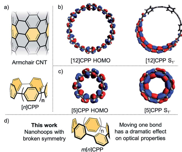
Fig. 1 (a) Structure of an armchair carbon nanotube (CNT) and its relation to [n] cycloparaphenylenes; (b) HOMO (left) and excited state (right) S_1 orbitals of [12]CPP and (c) HOMO (left) and excited state (right) S_1 orbitals of [5]CPP. Orbitals have been calculated using CAM-B3LYP/STO-3G level of theory. (d) meta [n] CPPs with broken symmetry in this work.
