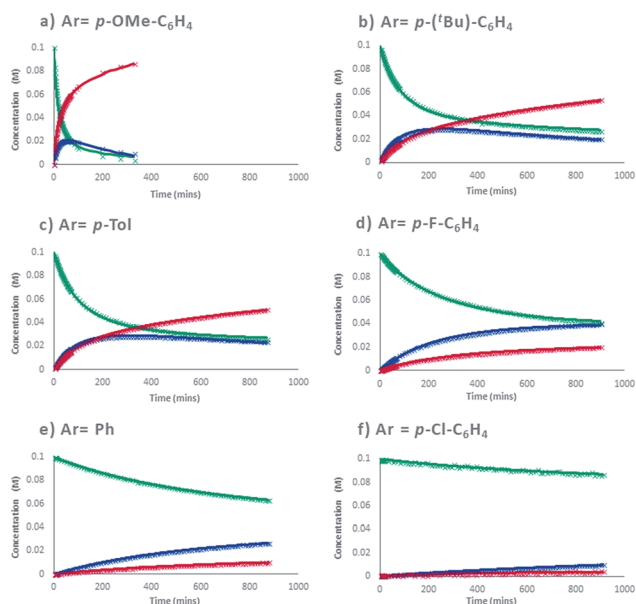
Scheme 8 Reaction progress with varying homoallylic alcohols.
