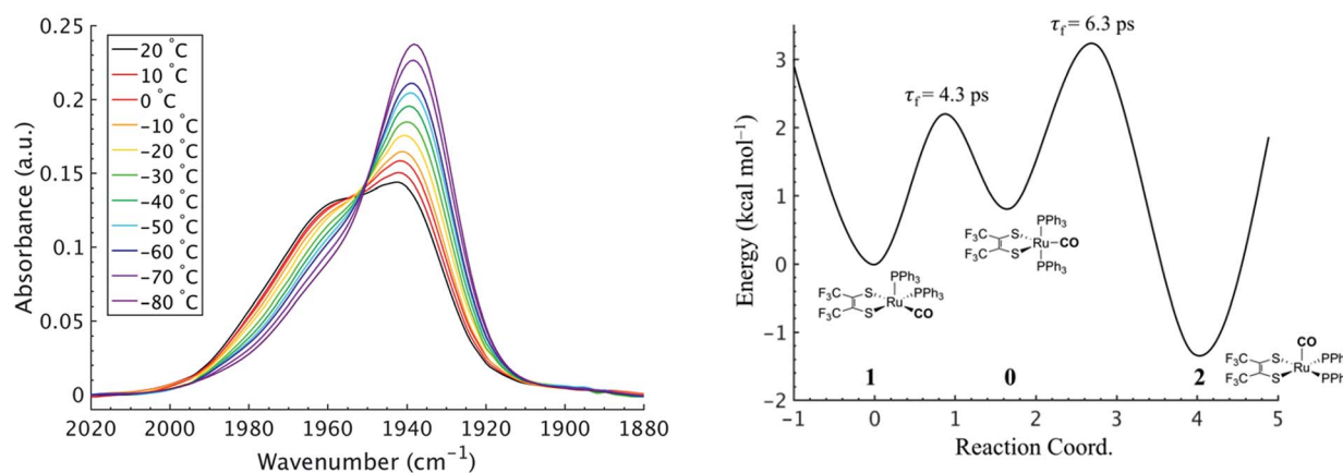
Fig. 3 (Left) VTFTIR of \text{Ru}(\text{S}_2\text{C}_2(\text{CF}_3)_2)_2(\text{CO})(\text{PPh}_3)_2 in DCM from 20 to -80^\circ\text{C} . (Right) Qualitative potential energy surface for the presented isomerization reaction. Energy surface was constructed using the experimental kinetic and thermochemical data obtained from 2D IR and VT-FTIR.
