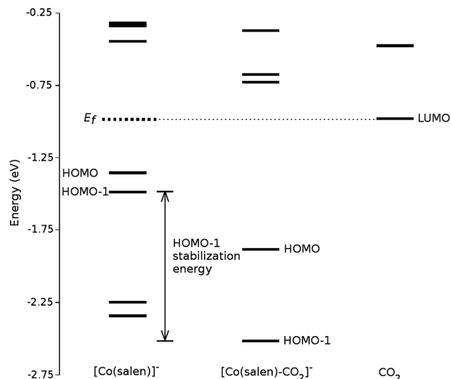
Fig. 8 Molecular orbital diagram of [\text{Co(salen)}]^- , [\text{Co(salen)-CO}_2]^- , and \text{CO}_2 . The figure shows the alignment of \text{CO}_2 LUMO with the Fermi energy of [\text{Co(salen)}]^- , explaining the possibility of back-donation and charge transfer.
