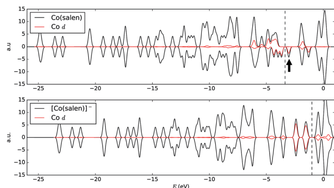
Fig. 9 Electronic density of states of (top) \text{Co(salen)} and (bottom) [\text{Co(salen)}]^- . The Fermi energy is indicated with a dashed line calculated directly from self-consistent field calculation. The Fermi energy increased from -3.325 eV to -1.0025 eV after the reduction of \text{Co(salen)} to [\text{Co(salen)}]^- complex, allowing the frontier orbitals to have good overlap with the \pi^* LUMO of the \text{CO}_2 molecule. Local density of Co d states are shown in red curve. The black arrow points to the polarized d state in the midgap region.
