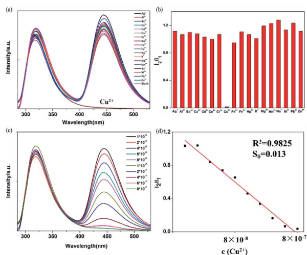
Fig. 6 (a) Fluorescence spectra of BBM-PMO-10 ( 5 \times 10^{-6} \text{ g mL}^{-1} ) with different metal ions ( 10^{-6} \text{ M} ) in \text{THF}/\text{H}_2\text{O} = 3 : 7 (v/v); (b) fluorescence intensity ratio I_2/I_1 of BBM-PMO-10 ( 5 \times 10^{-6} \text{ g mL}^{-1} ) with different metal ions ( 10^{-6} \text{ M} ) in \text{THF}/\text{H}_2\text{O} = 3 : 7 (v/v); (c) fluorescence spectra of BBM-PMO-10 in \text{THF}/\text{H}_2\text{O} = 3 : 7 (v/v) with different concentrations of \text{Cu}^{2+} ( 10^{-8} - 8 \times 10^{-7} \text{ M} ); (d) linear relationship between I_2/I_1 of BBM-PMO-10 ( 5 \times 10^{-6} \text{ g mL}^{-1} ) and the concentration of \text{Cu}^{2+} in the solvent.
