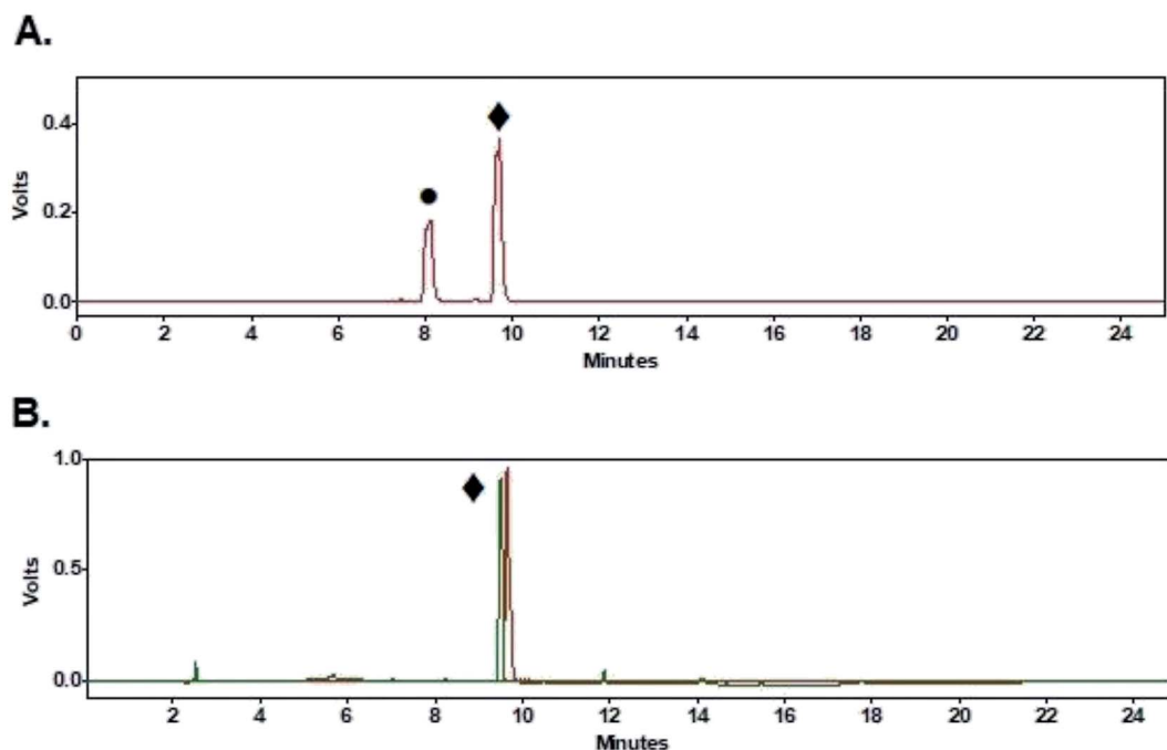
Fig. 6 HPLC chromatogram of radiolabeled [^{18}\text{F}]\text{FPy-YGGFL} (6) (PMT(gamma)-red, UV(220 nm)-green). (A) Crude radioHPLC chromatogram (peak \bullet -6- [^{18}\text{F}] fluoronicotinic acid, peak \blacklozenge - [^{18}\text{F}]\text{FPy-YGGFL} (6)). (B) Purified HPLC chromatogram co-injected with [^{19}\text{F}]\text{FPy-YGGFL} (peak \bullet -6- [^{19}\text{F}] fluoronicotinic acid, peak \blacklozenge - [^{19}\text{F}]\text{FPy-YGGFL} (6)).
