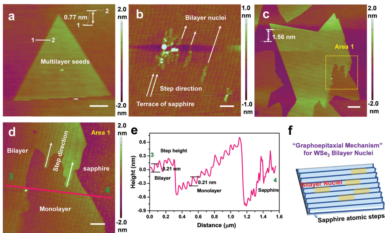
Fig. 2 (a and b) AFM topographic images of a monolayer WSe 2 crystal with bilayer nuclei in the center area. The inset height profile was ~0.8 nm, indicating a monolayer thickness of WSe 2 . The zoomed-in AFM image in b shows initial WSe 2 bilayer nuclei aligned growth on the atomic steps of sapphire. (c and d) AFM topographic images of bilayer WSe 2 crystals. The inset height profile in c was ~1.6 nm, indicating a bilayer thickness of WSe 2 . (e) The vertical profile was taken along the magenta line indicated in d (from 3 to 4). The average step height of sapphire terrace with monolayer/bilayer WSe 2 covering was ~0.2 nm. The small corrugation on the bare sapphire surface was 0.2–0.5 nm. (f) The proposed schematic of WSe 2 bilayer nuclei growth along the surface step nanogrooves of sapphire. The bilayer nuclei alignments on the atomic steps abide by the graphoeptitaxial mechanism. Scale bars: a, 2 μm; b, 200 nm; c, 500 nm; d, 200 nm.
