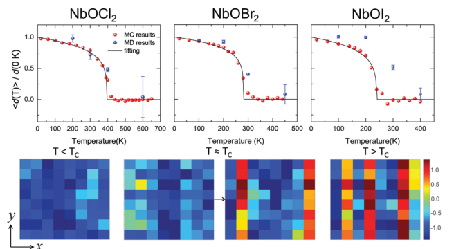
Fig. 7 Structural phase-transitions and Curie temperatures of NbOX 2 monolayers. Upper panel: Temperature dependence of the average Nb polar displacement obtained from MC and ab initio MD simulations for NbOCl 2 , NbOBr 2 and NbOI 2 monolayers. Average polar displacement \langle d(T) \rangle is normalized with respect to the corresponding 0 K value. Black lines are fitted to MC data based on eqn (3). The error bars of Nb polar displacement highlight the thermal fluctuations during the MD simulations. Lower panel: MD simulated polarization reversal process in NbOI 2 monolayer. The normalized polar displacements ( d_i(T)/d_i(0 \text{ K}) ) for each Nb cation in a 8 × 8 lattice grid are presented when the temperature is below, approaching and above Curie temperature T_C . Polarization reversal occurs when T \approx T_C , and is initiated by switching d_i of a single Nb from one cation column along the polar axis ( y direction).
