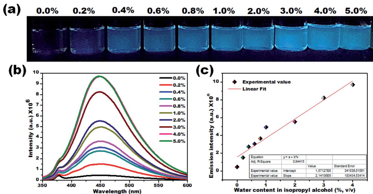
Fig. 5 Visual colorimetric water sensing performance of CD1 on hydrated protic isopropyl alcohol. (a) Photograph of CD1 in IPA and hydrated IPA with varied water content (0.2% to 5.0% v/v) under UV light ( \lambda_{\text{max}} = 365 nm), and (b) their corresponding PL emission spectra ( \lambda_{\text{ex}} = 330 nm). The gradual enhancement in the emission intensity was noted upon increasing the water content in isopropyl alcohol. (c) Calibration curve (percentage of water content vs. emission intensity).
