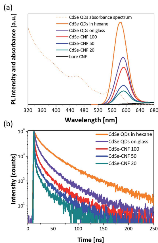
Fig. 5 (a) Absorbance and PL spectra of the synthesized CdSe QDs dispersed in hexane and PL spectra of CdSe–CNFs and a CdSe QD layer on glass. (b) Transient PL decay curves of CdSe QDs in hexane, a CdSe QD layer on glass, and CdSe–CNFs. Every characterization is performed using a source of light (excitation wavelength = 470 nm). For the CdSe QD film on glass, the CdSe QDs (20 mg mL −1 in hexane) were spin coated on glass at 2000 rpm for 30 s.
