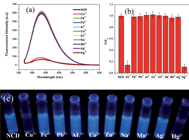
Fig. 4 (a) Fluorescence emission spectra of NCDs (2 mL) in the presence of different metal ions ( \lambda_{\text{ex}} = 360 \text{ nm} , [\text{M}^{n+}] = 50 \text{ }\mu\text{M} , 10 \text{ }\mu\text{L} ); (b) bar diagram of relative fluorescence emission intensities ( F/F_0 ) of NCDs in the presence of different metal ions; (c) image of fluorescence sensing experiment with NCDs for different metal ions under 365 nm UV lamp.
