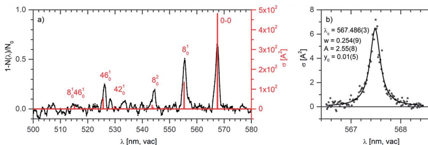
Fig. 5 (a) Helium tagging visPD spectrum of \text{C}_{14}\text{H}_{10}^{2+} generated by electron ionization from anthracene measured with a Sunlite laser (see Experimental details). The red spectrum was calculated using the Franck–Condon harmonic approximation, and the 0–0 band position was set to the experimental value. (b) Details of the 0–0 transition band in the helium tagging visPD spectrum of \text{C}_{14}\text{H}_{10}^{2+} . The parameters are characteristics of the Lorentzian fit. The Sunlite laser fluence was 0.7 \text{ mJ cm}^{-2} . For details of the absolute cross section determination see the ESI.†
