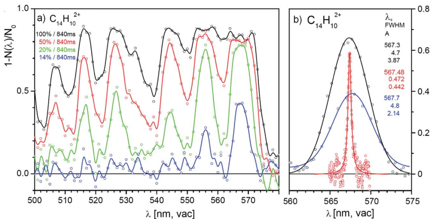
Fig. 4 (a) Helium tagging visPD spectrum of C_{14}H_{10}^{2+} generated by electron ionization from anthracene. The spectra were recorded with different laser power levels (black: 100%; red: 50%; green: 20%; blue: 14%). (b) Comparison of line shapes measured under different conditions and with different laser sources. Blue: SuperK laser focused with lens; black: SuperK laser beam directly from the laser output; red: Sunlite laser. The numbers correspond to the indicated characteristics of the Gaussian (black and blue) and Lorentzian fits.
