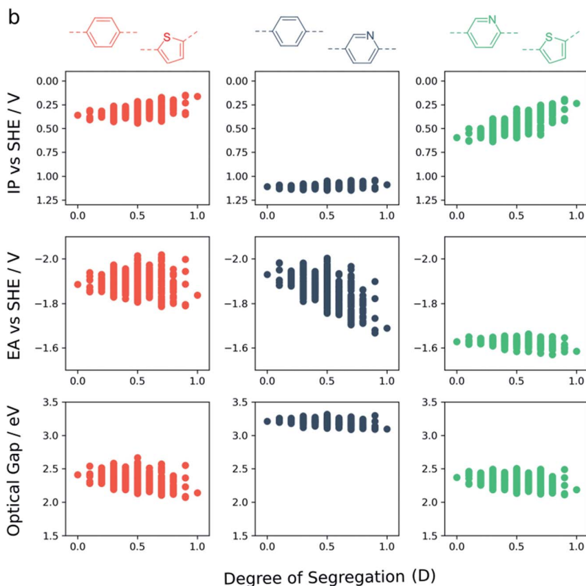
Fig. 5 (a) Schematic of how the 'degree of segregation' ( D ) is measured: the number of equivalent neighbouring monomer units within a given sequence isomer ( n ), divided by the total number of monomer units ( N ) minus 2. This metric spans values between 0 (fully alternating) and 1 (fully segregated into a block of monomer A and a block of monomer B). (b) Illustration of how the 'degree of segregation' of co-monomers influences the overall co-polymer properties (IP, EA and optical gap) for 1 : 1 co-polymers.
