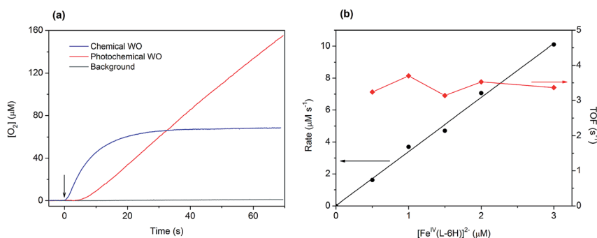
Fig. 3 (a) Traces of oxygen evolution obtained in photochemical (red trace: [\text{Fe}^{\text{IV}}(\text{L}-6\text{H})]^{2-} ( 1\text{ }\mu\text{M} ), [\text{Ru}(\text{bpy})_3]^{2+} ( 0.2\text{ mM} ) and \text{S}_2\text{O}_8^{2-} ( 2\text{ mM} )) and chemical water oxidation experiments (blue trace: [\text{Fe}^{\text{IV}}(\text{L}-6\text{H})]^{2-} ( 1.5\text{ }\mu\text{M} ) and [\text{Ru}(\text{bpy})_3]^{3+} ( 1\text{ mM} )). Oxygen evolution in the absence of catalyst is given for comparison (grey trace: [\text{Ru}(\text{bpy})_3]^{2+} ( 0.2\text{ mM} ) and \text{S}_2\text{O}_8^{2-} ( 2\text{ mM} )). The arrow indicates the beginning of the reaction (the start of illumination or addition of the oxidant, respectively). (b) Initial water oxidation rates (circles) and TOF (diamonds) as a function of the catalyst concentration for chemical water oxidation using [\text{Ru}(\text{bpy})_3]^{3+} ( 1\text{ mM} ).
