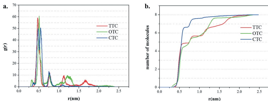
Fig. 10 (a) The radial distribution function (RDF) of the three TC molecules on the GO surface; (b) the running coordination numbers of the three TCs to the surface of GO.
