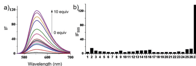
Fig. 85 (a) Fluorescent emission spectra of 10 \mu\text{M} probe 55 in the presence of 0–10 equiv. of \text{H}_2\text{S} in aqueous solution ( \text{CH}_3\text{CN}/\text{PBS} = 1:9 , pH = 7.4, 37^\circ\text{C} ) (NaHS was dissolved in water at a concentration of 10 \text{ mM} ). Excitation at 450 nm. (b) Fluorescence responses of 10 \mu\text{M} 55 to various analytes in aqueous solution ( \text{CH}_3\text{CN}/\text{PBS} = 1:9 , pH = 7.4, 37^\circ\text{C} ). Excitation at 450 nm. Bars represent the final fluorescence intensity of 55 with 1 \text{ mM} analytes over the original emission of free 55 . (1) Free 55 ; (2) \text{Zn}^{2+} ; (3) \text{Na}^+ ; (4) \text{Ca}^{2+} ; (5) \text{K}^+ ; (6) \text{Mg}^{2+} ; (7) \text{HCO}_3^- ; (8) \text{F}^- ; (9) \text{Cl}^- ; (10) \text{Br}^- ; (11) \text{I}^- ; (12) \text{NO}_3^- ; (13) \text{S}_2\text{O}_3^{2-} ; (14) \text{S}_2\text{O}_4^{2-} ; (15) \text{S}_2\text{O}_5^{2-} ; (16) \text{SO}_3^- ; (17) \text{N}_3^- ; (18) \text{CO}_3^{2-} ; (19) \text{CH}_3\text{COO}^- ; (20) \text{SO}_4^{2-} ; (21) \text{H}_2\text{O}_2 ; (22) \text{HSO}_4^- ; (23) homocysteine; (24) ascorbic acid; (25) cysteine; (26) glutathione; and (27) NaHS. Copyright 2013 American Chemical Society.
