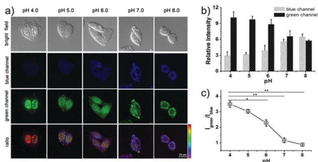
Fig. 62 (a) Fluorescence images for 5 \mu\text{M} 41 in HeLa cells at various pH values: blue channel, emission at 425–475 nm with excitation at 405 nm; green channel, emission at 500–550 nm with excitation at 488 nm. Ratio images represent the ratio of fluorescence intensity between the green channel and blue channel ( I_{\text{green}}/I_{\text{blue}} ). (b) Quantified relative fluorescence intensity at various pH values was analyzed using Nikon NIS Element software and presented as mean \pm SD, with n = 3 . (c) Ratio of I_{\text{green}}/I_{\text{blue}} at various pH values obtained from panel b. Statistical analyses were performed with Student's t test ( n = 3 ). * P < 0.05 , ** P < 0.01 , and error bars are \pm SD. Copyright 2016 American Chemical Society.
