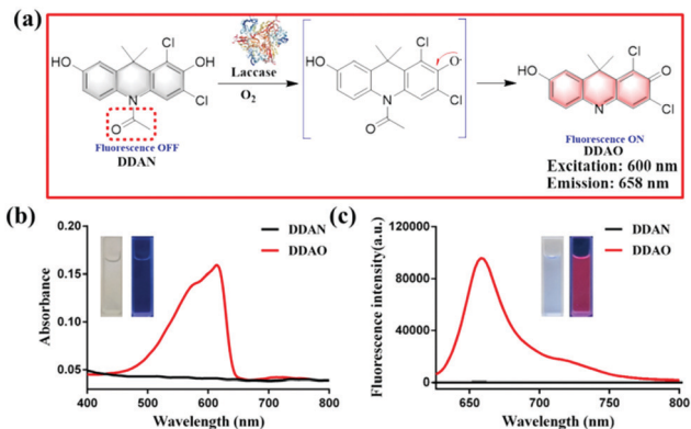
Fig. 1 (a) Proposed mechanism of the sensing of fungal laccase using DDAN . (b) Absorbance spectra of DDAN and DDAO . (c) Fluorescence spectra of DDAN and DDAO ( \lambda_{\text{ex}} = 600 nm).
