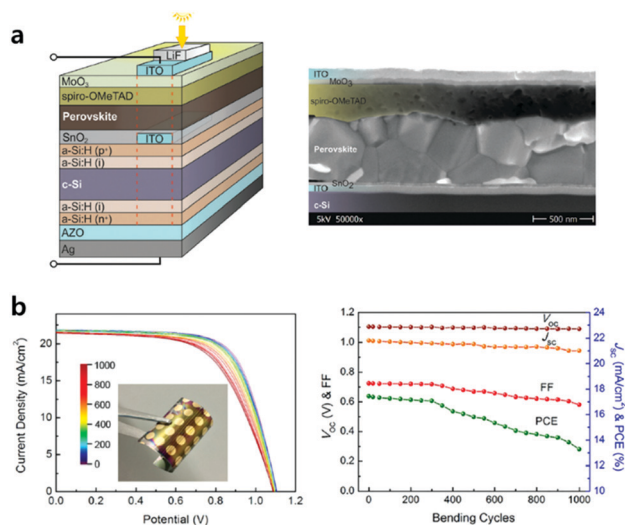
Fig. 7 (a) Schematic of the Si heterojunction/perovskite tandem solar cell (the red dashed line indicates the active area) and cross-sectional scanning electron micrograph of a typical monolithic tandem solar cell. Reproduced with permission. 65 Copyright 2016, The Royal Society of Chemistry. (b) Fatigue testing of a flexible PSC with a bending radius of 1 cm. J - V curves measured after various bending cycles and performance parameters as a function of bending cycles. Reproduced with permission. 59 Copyright 2017, American Chemical Society.
