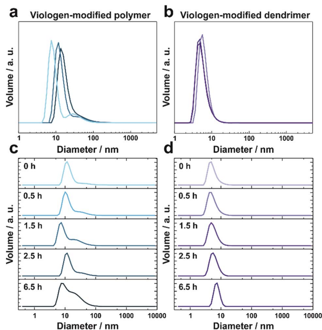
Fig. 2 Size distributions of viologen-modified dendrimers and polymers. Dynamic light scattering measurements of (a) viologen-modified polymer and (b) viologen-modified dendrimer under anaerobic conditions. The three replicates were from three individual preparations under the same conditions. (c) Viologen-modified polymer and (d) viologen-modified dendrimer after various incubation times (as indicated in the figure) in ambient air. The concentrations of the polymer and dendrimer are 0.25 \text{ mg mL}^{-1} and 1 \text{ mg mL}^{-1} , respectively. DLS data are presented as distribution by volume. All measurements were performed in Tris buffer solution (100 mM, pH 9.0), in the presence of tris(2-carboxyethyl)phosphine (TCEP, 1.25 mM).
