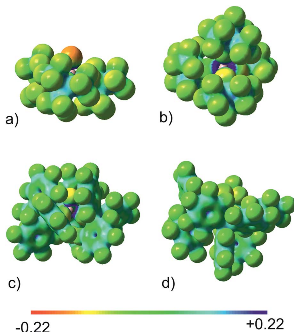
Fig. 5 Projection of the calculated electrostatic potential on the 0.025 e − bohr −3 isodensity surface. (a) [FAI(OC(CF 3 ) 3 ) 3 ] − ; (b) [Al(OC(CF 3 ) 3 ) 4 ] − ; (c) [FAI(OCArF 3 ) 3 ] − ; (d) [CIAI(OCArF 3 ) 3 ] − . B3LYP/6-311++G(2d,2p) level of theory.
