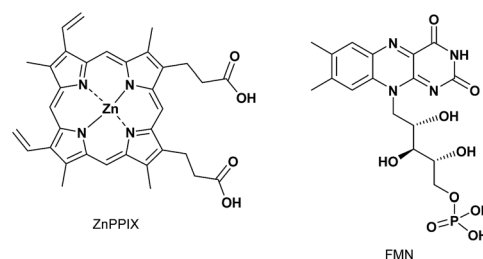
Scheme 5 Structures of ZnPPIX and FMN.
