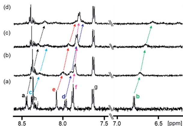
Fig. 2 Partial ^1\text{H} NMR spectra (500 MHz) of 1 in the absence and presence of PPIX in \text{DMSO-}d_6 /33 mM HEPES buffer (pD 7.4) = 2 : 1 (v/v) at 23 °C. (a) 1 (0.10 mM), (b) 1 (0.10 mM) + PPIX (0.020 mM), (c) 1 (0.10 mM) + PPIX (0.050 mM) and (d) 1 (0.10 mM) + PPIX (0.10 mM). 1% tetramethylsilane in \text{CCl}_4 was used as the external reference. Peak assignments of aromatic protons \text{H}^a\text{--H}^i on 1 are listed in Scheme 3.
