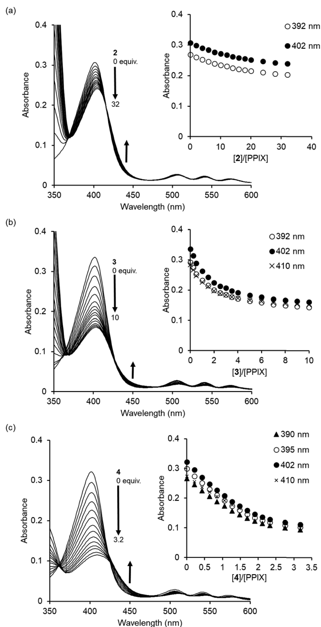
Fig. 3 UV-Vis titrations of PPIX (2.4 \mu\text{M} ) with (a) 2 , (b) 3 , and (c) 4 in \text{DMSO} /33 mM HEPES buffer (pH 7.4) = 2 : 3 (v/v) at 25 °C. Insets: changes in the absorbance of PPIX upon the addition of compounds 2–4.
