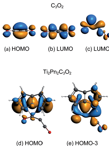
Fig. 8 Key orbitals of linear and bent \text{C}_3\text{O}_2 and \text{Ti}_2\text{Pn}_2\text{C}_3\text{O}_2 .
