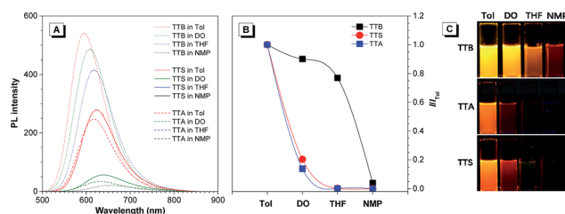
Fig. 1 (A) Emission spectra of TTB, TTS, and TTA in solvents with different polarities. Concentration: 10 \mu\text{M} ; excitation wavelength: 480 nm. (B) Relative PL intensity ( I/I_{Tol} ) of TTB, TTA, and TTS in different solvents, where I_{Tol} = PL intensity in toluene and I = PL intensity in other solvents. (C) Fluorescence photographs of TTB, TTA, and TTS in different solvents taken under 365 nm UV illumination.
