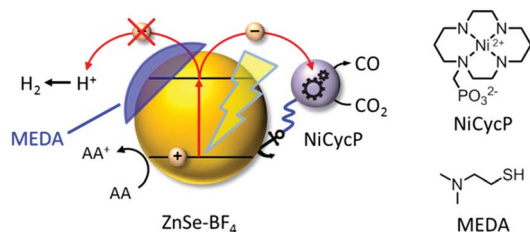
Fig. 1 Schematic representation of the photocatalyst system developed in this work: ligand-free ZnSe QDs (ZnSe-BF 4 ) combined with a molecular electrocatalyst, NiCycP, for aqueous CO 2 reduction to CO. H 2 evolution can be partially suppressed by a surface inhibitor (MEDA). AA: ascorbic acid.
