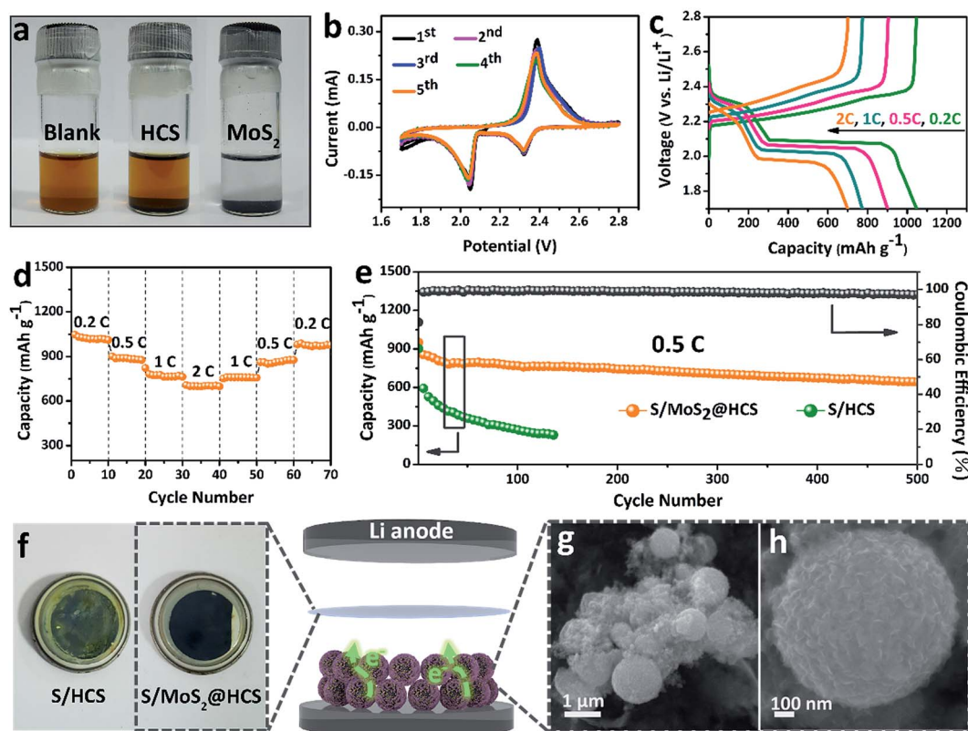
Fig. 3 (a) Polysulfide entrapment by the HCSs and \text{MoS}_2 nanosheets. (b) CV curves of the \text{S}/\text{MoS}_2@ HCS composite electrode at a scan rate of 0.1 \text{ mV s}^{-1} . (c) Voltage profiles and (d) rate capacities of the \text{S}/\text{MoS}_2@ HCS composite electrode at various current densities ranging from 0.2 to 2C. (e) Prolonged cycling performance of the \text{S}/\text{MoS}_2@ HCS composite and \text{S}/\text{HCS} electrodes at 0.5C. (f) The separator of the \text{S}/\text{HCS} and \text{S}/\text{MoS}_2@ HCS composite after the 100th cycle in the voltage range 1.7–2.8 V. (g and h) FESEM images of the \text{MoS}_2@ HCS composite after cycling.
