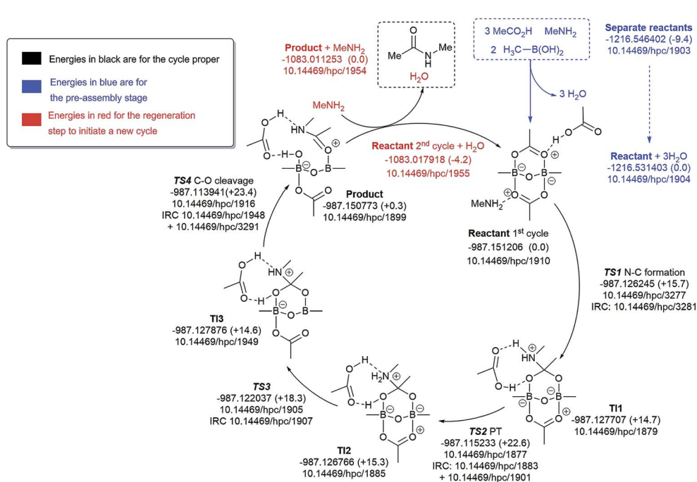
Fig. 9 Catalytic cycle involving one amine (data 29 sub-collection DOI: 10.14469/hpc/1854). The total computed free energy for each stationary point is shown in Hartree, with the relative energies shown in parentheses in kcal mol ^{-1} . The DOI for data repository entries for individual species are shown in the form e.g. 10.14469/hpc/1885. Energies in blue are for the pre-assembly stage, in black for the cycle proper and in red for the regeneration step to initiate a new cycle. All DOIs in this figure are available as clickable links (final paginated PDF only).
