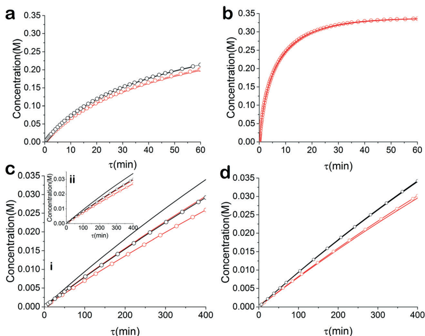
Fig. 7 Simulated kinetic data of esterification reaction with simultaneous temperature and residence time ramps. Kinetic data at — 30 °C, — 60 °C. Fitted model at — 30 °C, — 60 °C. (a) Control example in terms of reaction rate and ramp rates. (b) Fast reaction example with control ramp rates (c) slow reaction with i) control temperature and residence time ramp rates and ii) control temperature ramp rate and slow residence time ramp rate (d) slow reaction with slow temperature ramp rate and slow residence time ramp rate.
