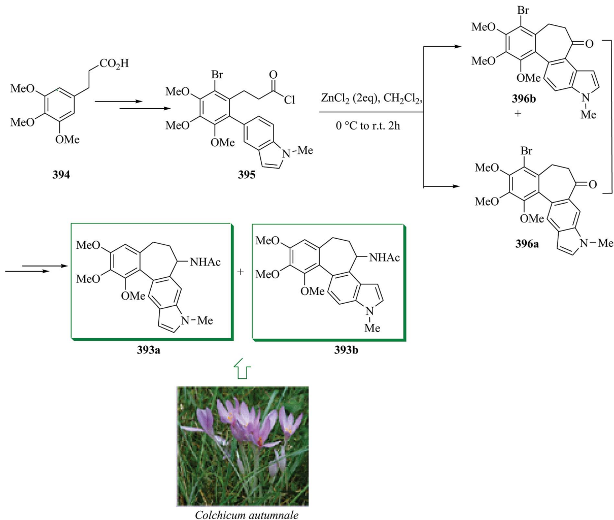
Scheme 83 Total synthesis of allocolchicinoids rac - 393a and rac - 393b .
