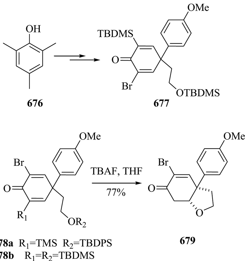
Scheme 146 The formation of the bicyclic compound 679 .
