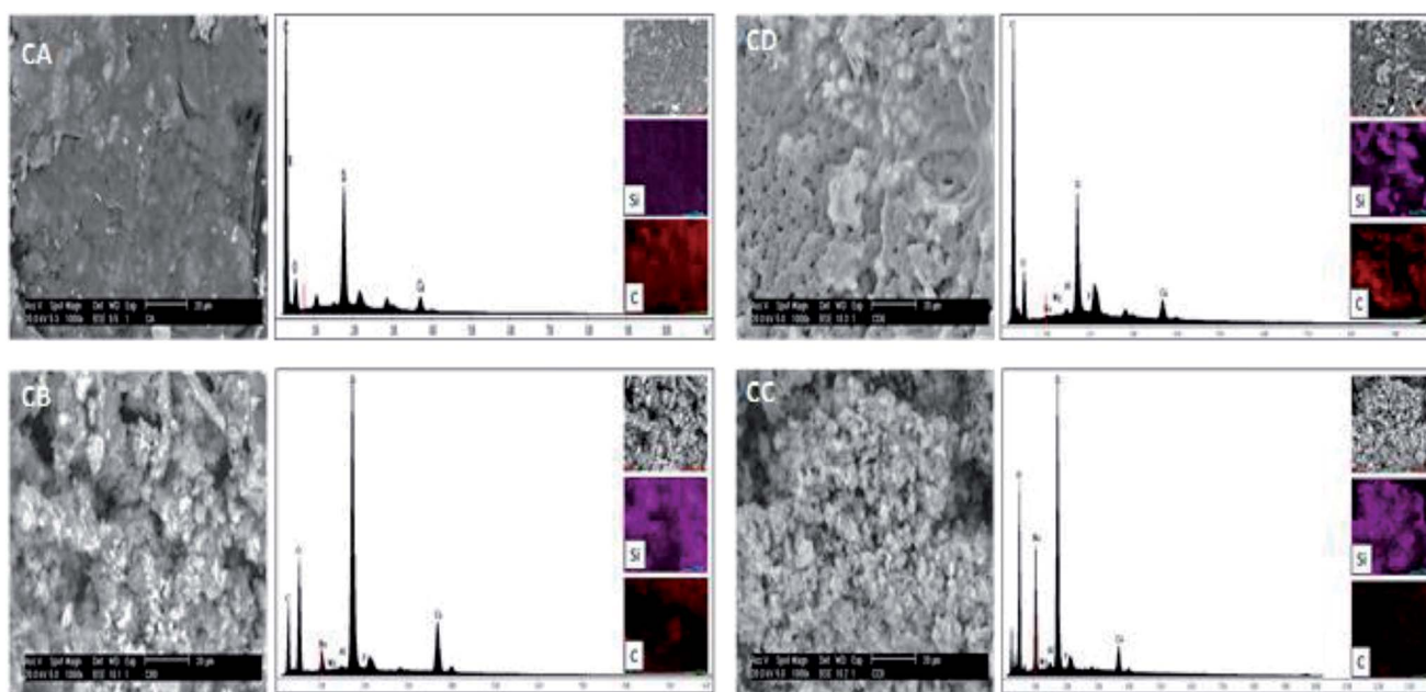
Fig. 8 SEM micrographs, energy spectra and element mapping images of Si and C of the samples CA, CB, CC and CD.
