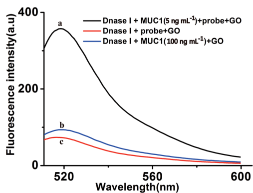
Fig. 2 The feasibility analysis. (a) Dnase I + MUC1 (5 ng mL -1 ) + probe + GO; (b) Dnase I + MUC1 (100 ng mL -1 ) + GO; (c) Dnase I + probe + GO. The concentrations of Dnase I, GO and probe were 2 U mL -1 , 15 μg mL -1 and 40 nM, respectively.
