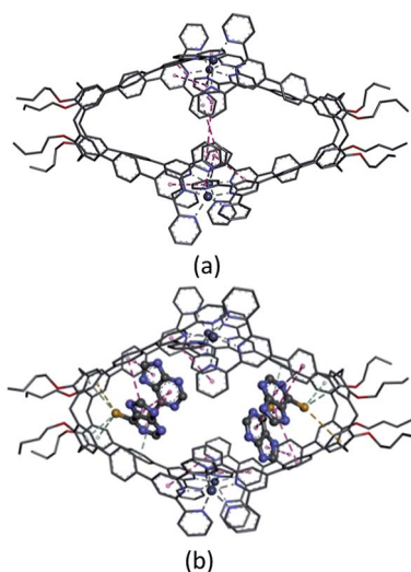
Fig. 4 The optimized structures of \text{Zn}_4\text{L1}_2 (a) and 4(\text{mercaptapurine})@ \text{Zn}_4\text{L1}_2 (b). The interactions are colored in dotted lines: coordination bond in gray, S- \pi interaction in green, S-H- \pi interaction in yellow and \pi - \pi interaction in pink. All hydrogens are omitted for clarity.
