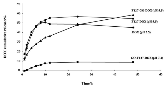
Fig. 4 The release percentage curves of DOX from the F127-GO-DOX hydrogel ( \Delta , pH 5.5; \blacksquare , pH 7.4), F127-DOX hydrogel ( \bullet ), and DOX solution ( \blacklozenge ).
