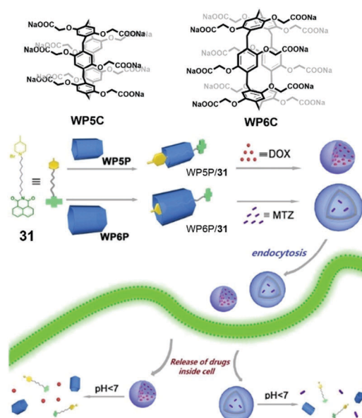
Fig. 24 Chemical structures of WP5P, WP6P and pyridinium guest 31, and a cartoon representation of the self-assembling and controlled release processes. Adapted with permission from ref. 97. Copyright 2016 American Chemical Society.
