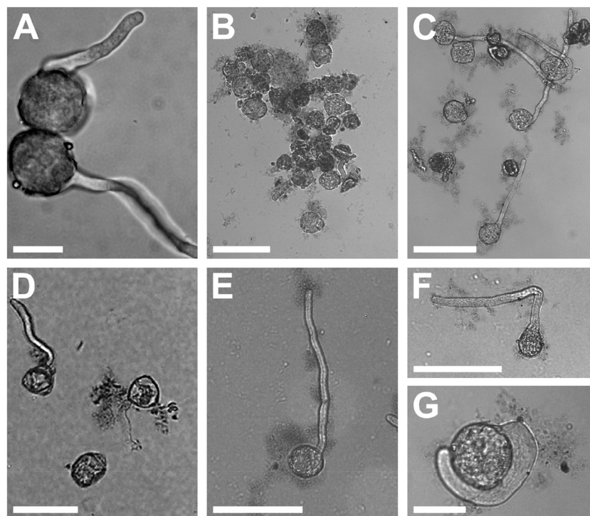
Fig. 2 Pollen of N. tabacum in BK PEG after 1 h (A), BK suc (B) or BK PEG (C) at 100 \mu\text{g GO mL}^{-1} after 2 h. Pollen of C. avellana in BK suc at 50 \mu\text{g GO mL}^{-1} after 5.5 h (D). Straight (E) or bent (F and G) grown pollen tubes of N. tabacum at 100 \mu\text{g GO mL}^{-1} . Bars: A, G = 20 \mu\text{m} ; D = 50 \mu\text{m} ; B, C, E, F = 100 \mu\text{m} .
