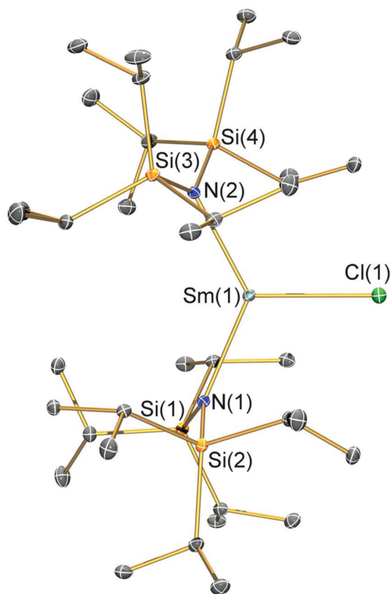
Fig. 2 Molecular structure of [\text{Sm}(\text{N}^+)_{2}(\text{Cl})] ( 2-Cl ) with selective atom labelling. Displacement ellipsoids set at a 30% probability level and hydrogen atoms are omitted for clarity. Selected bond lengths [Å]: Sm(1)–Cl(1) 2.5813(7), Sm(1)–N(1) 2.295(2), and Sm(1)–N(2) 2.317(2). Selected bond angles [°]: N(1)–Sm(1)–N(2) 128.24(7), N(1)–Sm(1)–Cl(1) 111.34(6), and N(2)–Sm(1)–Cl(1) 117.11(5).
