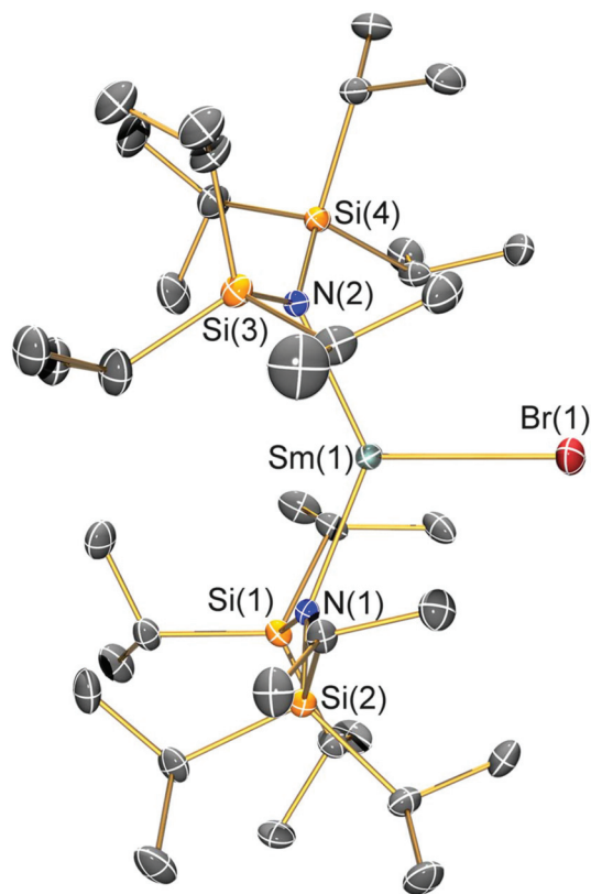
Fig. 3 Molecular structure of [\text{Sm}(\text{N}^+)_{2}(\text{Br})] ( 2-Br ) with selective atom labelling. Displacement ellipsoids set at a 30% probability level and hydrogen atoms are omitted for clarity. Selected bond lengths [Å]: Sm(1)–Br(1) 2.7429(7), Sm(1)–N(1) 2.308(4), and Sm(1)–N(2) 2.324(4). Selected bond angles [°]: N(1)–Sm(1)–N(2) 133.52(14), N(1)–Sm(1)–Br(1) 112.19(10), and N(2)–Sm(1)–Br(1) 113.19(10).
